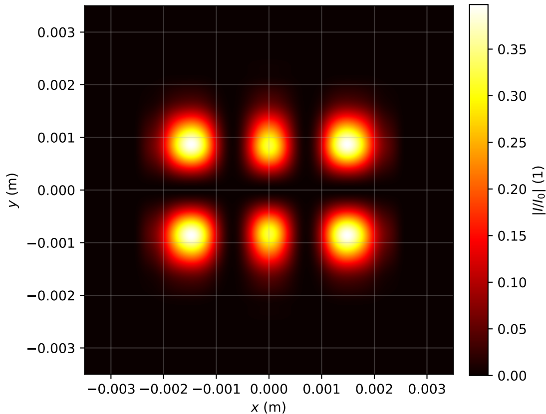
Intensity profile I(x, y, z = 3.184)/I_0 , P_{in}=2.0P_{cr} , artificial time
